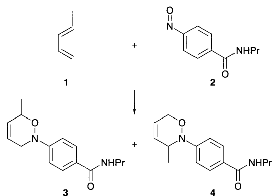
Scheme 1 Reaction between 1 and 2 carried out in PBS–5% Me 2 SO at room temp.; yields: 3 , 58%; 4 , 42%
